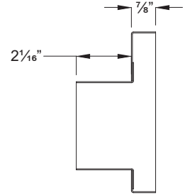
Square/Rectangular Collar Detail
