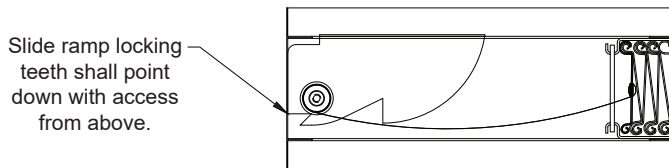
Open Position (30SH or 30DH)
